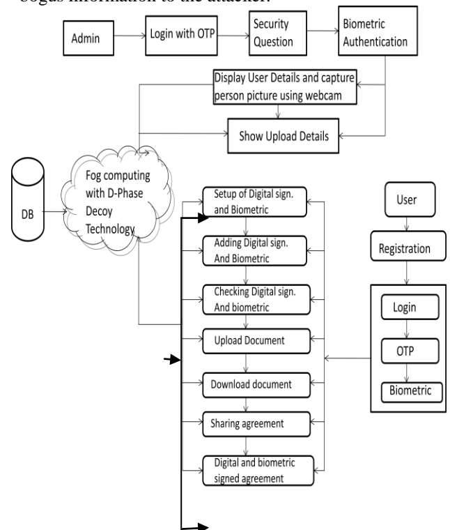
Fig. 3 System Architecture
