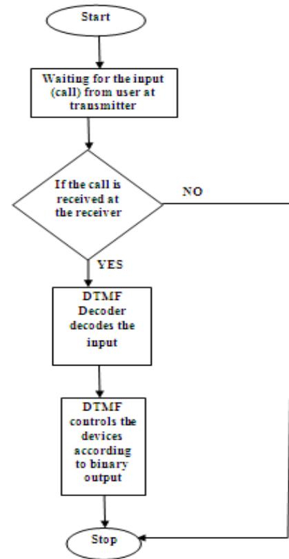
Figure7: flowchart determining DTMF based automation
