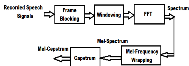
Figure-1: MFCCs feature extraction process.
